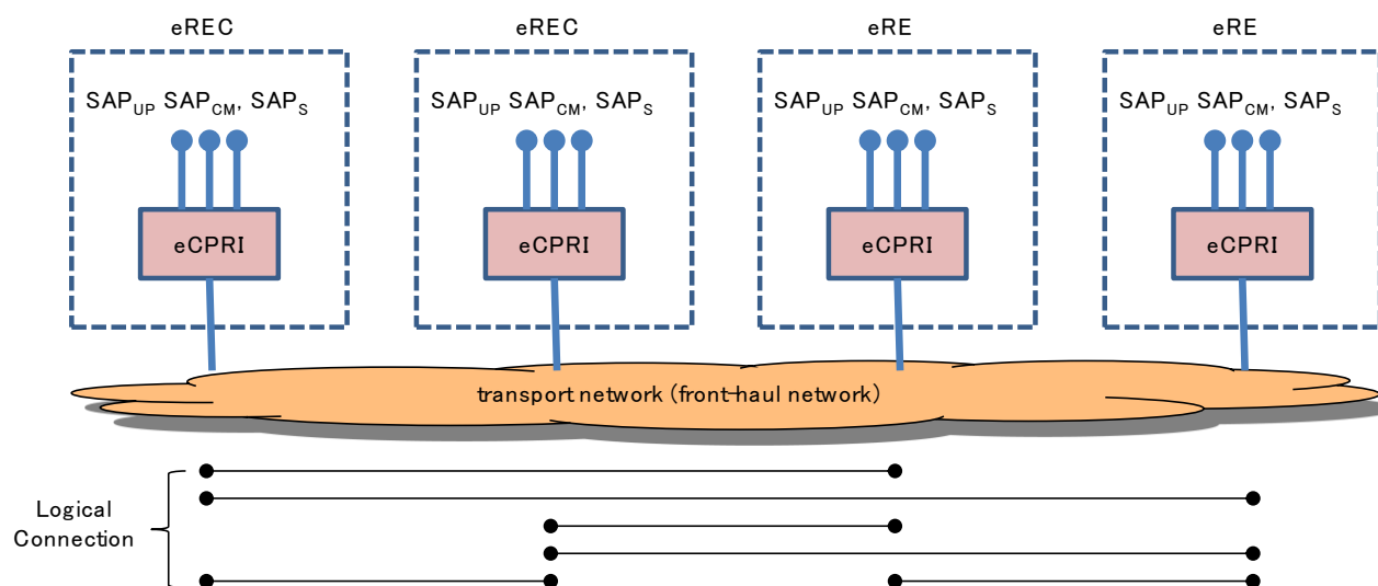
9 10 Figure 40: Network by eCPRI
