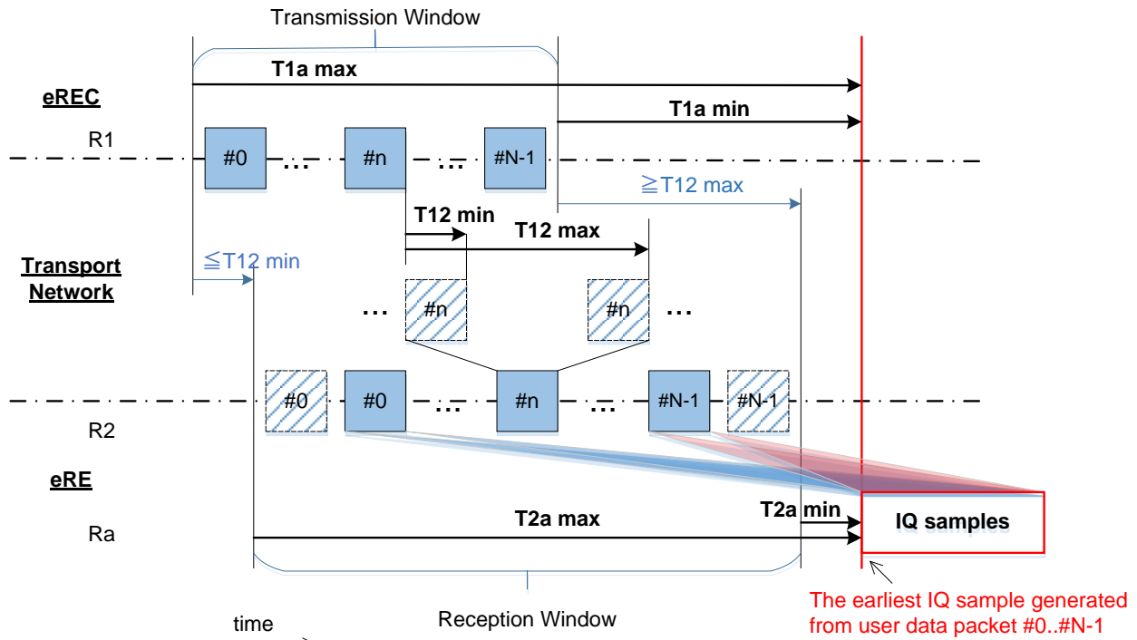
1 2 3 4 5 6 7 8 9 10 11 12 13 14 15 16 17 Figure 35: Timing relations in DL direction
