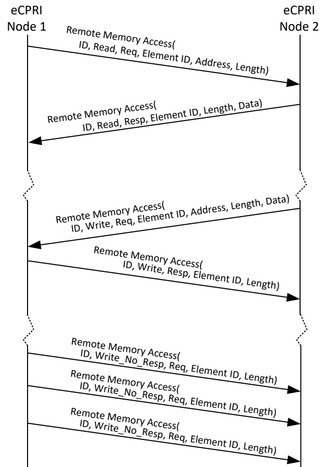
Figure 21: Message sequence diagram (example)
