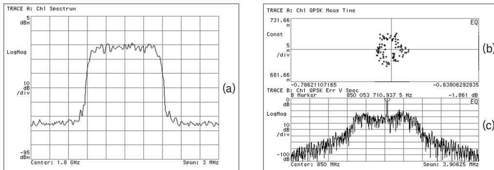
Figure 13. In-channel interfering tone not visible in (a) the frequency domain, but detectable in (b) the constellation and (c) error vector spectrum
