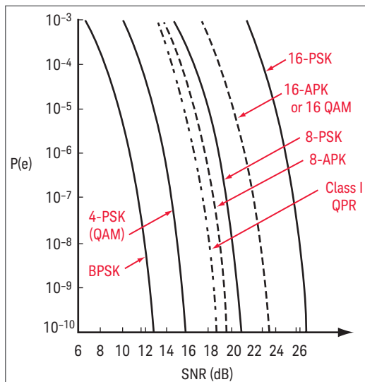
Figure 3. Probability of Error Versus SNR
