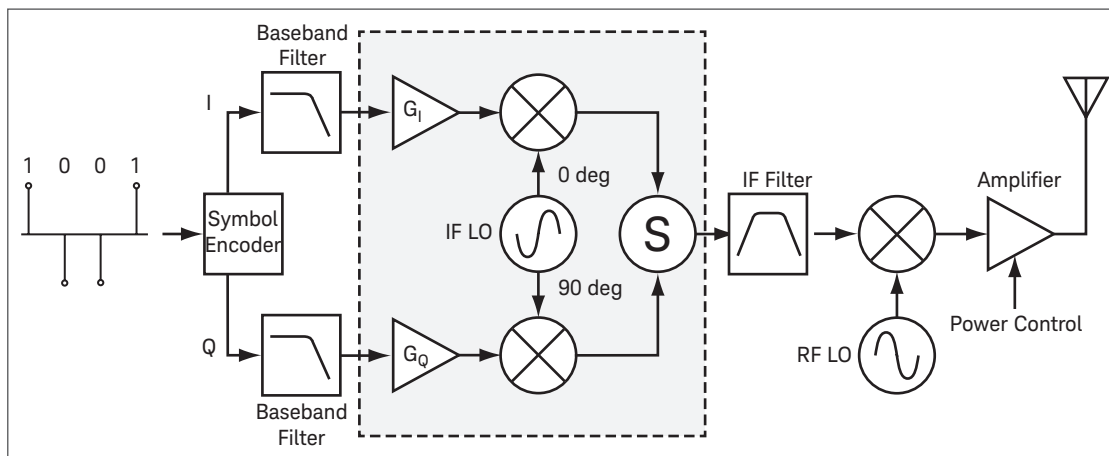
Figure 6. I/Q modulator
