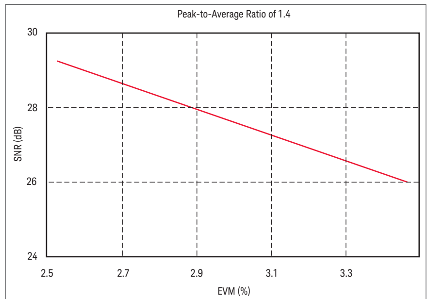
Figure 4. SNR versus EVM for crest factor of 1.4
