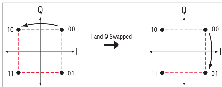
Figure 9. I/Q swapped
