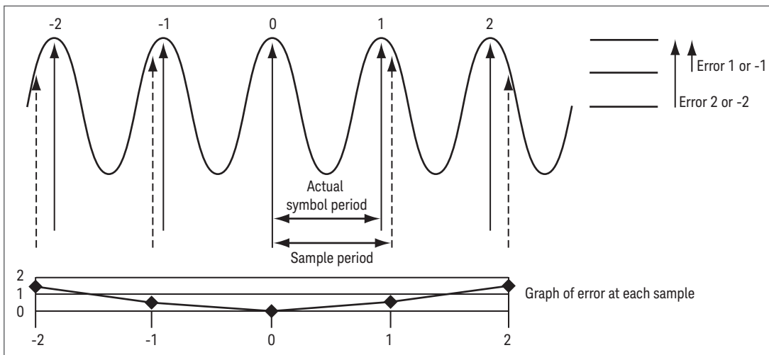
Figure 11. Symbol rate slightly higher than specified.
