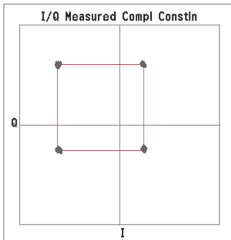
Figure 8. I/Q offsets
