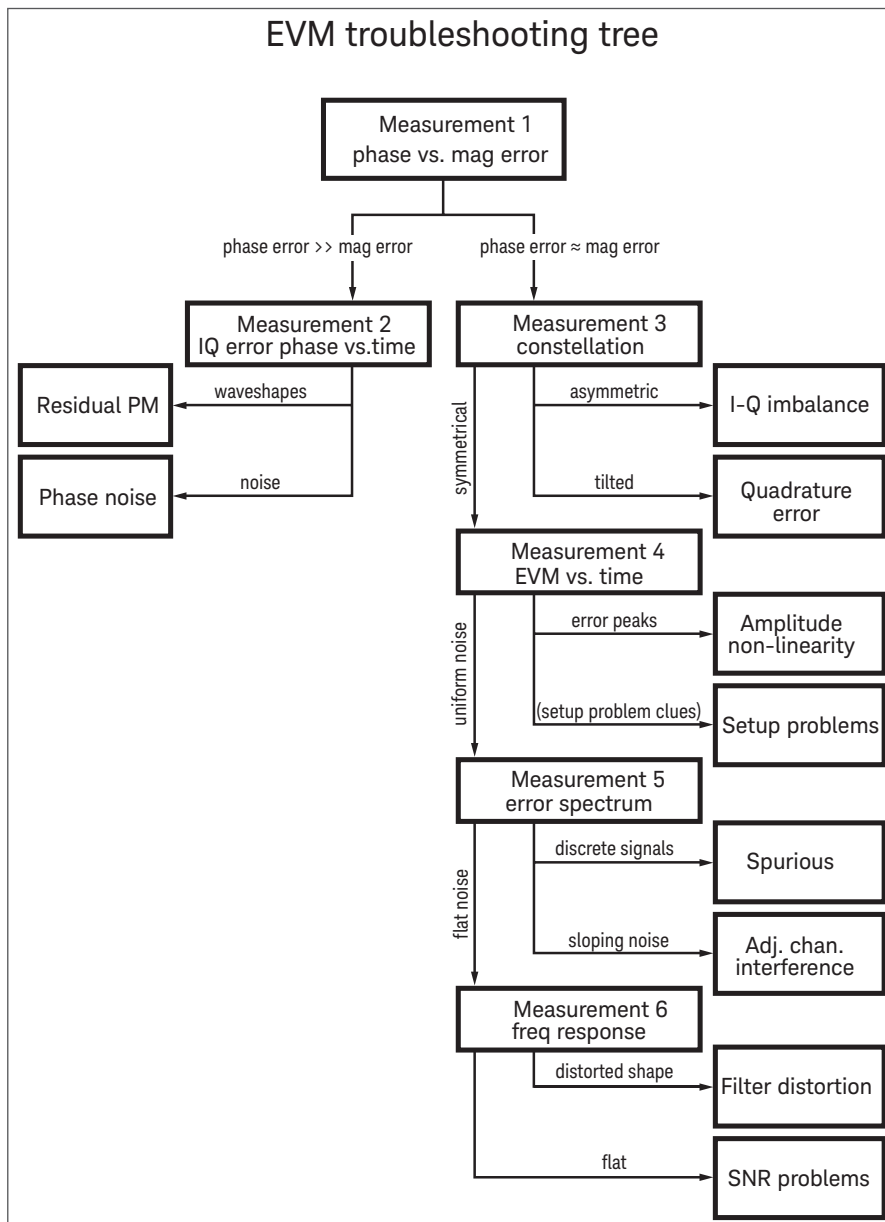
Figure 2. Flow chart for analyzing vector modulated signals with EVM measurements
