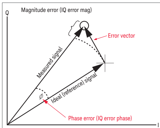
Figure 1. Error vector magnitude (EVM) and related quantities
