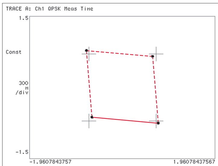
Figure 7. Quadrature error
