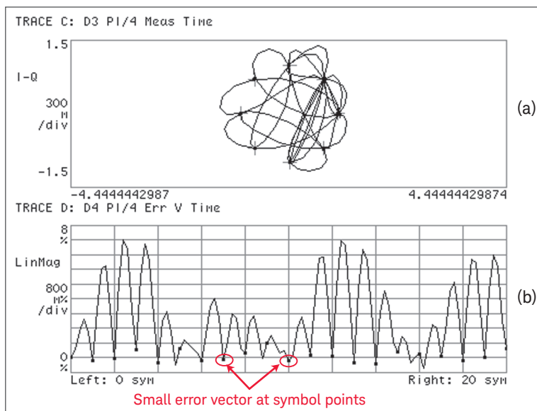
Figure 12. (a) Polar diagram and (b) magnitude of the error vector versus time for incorrect alpha. The error vector is large between symbol points and small at the symbol points
