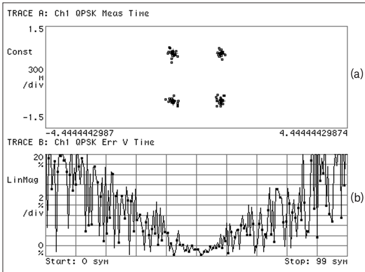
Figure 10. (a) Constellation and (b) magnitude of the error vector versus time with ‘V’ shape caused by incorrect symbol rate
