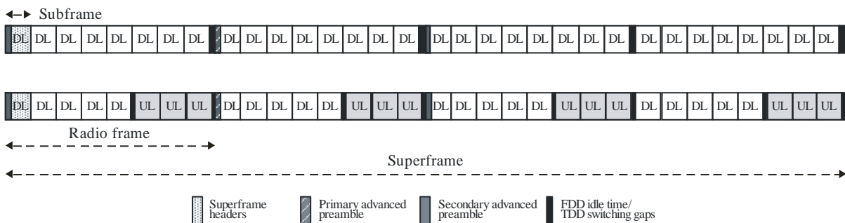
FIGURE 2.6 Structure of advanced preambles
