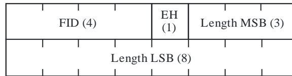
Advanced generic MAC headers
