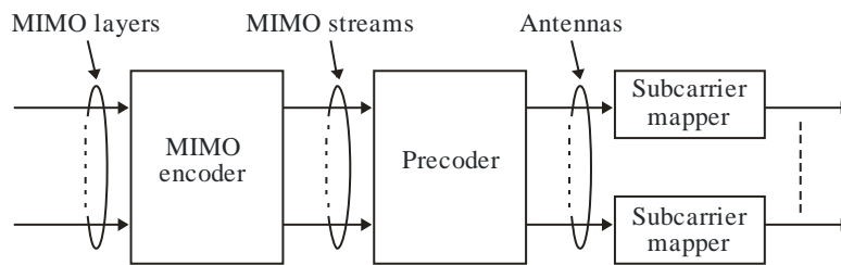
MIMO structure
